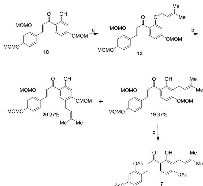
Scheme 2. a) Prenyl bromide, K_2CO_3 , acetone, reflux, 24 h, 95%; b) Montmorillonite K-10, CH_2Cl_2 , 0^\circ C , 8 h, 19 (37%), 20 (27%) and recovered 18 (33%); c) 1. conc. HCl, MeOH, RT, 20 h; 2. 4 M NaOH, RT, 2 h; 3. Ac_2O , pyridine, CH_2Cl_2 , RT, 12 h, 35% for two steps. MOM = methoxymethyl.
