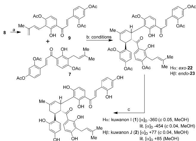
Scheme 3. a) SOCl_2 , DBU, CH_2Cl_2 , -78^\circ C to RT, 12 h, 75%; b) Ligand, BH_3 \cdot THF , AcOH, 5 Å M.S., THF, RT, 72 h; c) K_2CO_3 , MeOH/ H_2O (10:1), RT, 1 h, 70%. DBU = 1,8-diazabicyclo[5.4.0]undec-7-ene.
